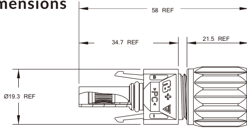
H4 Stamped and Formed Contact
