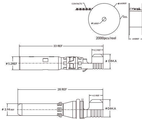
H4 Stamped and Formed Contact
