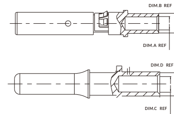
H4 Cold Formed Contact
